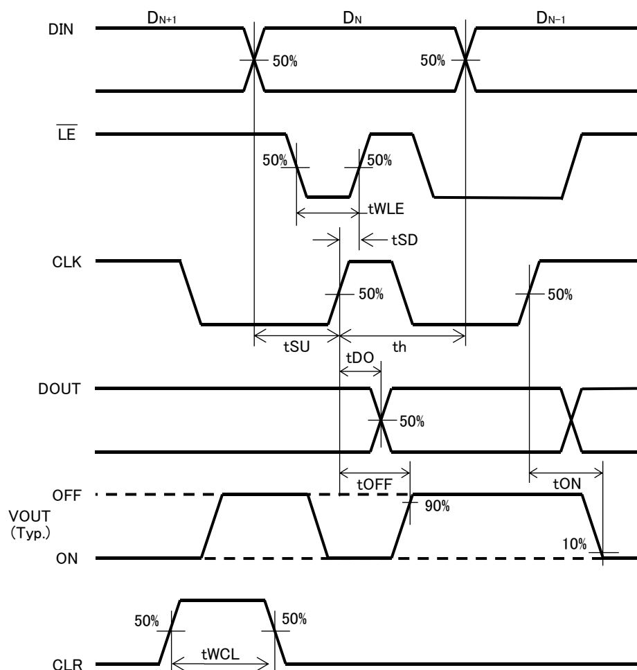
Fig. 5.1 Timing Waveforms
