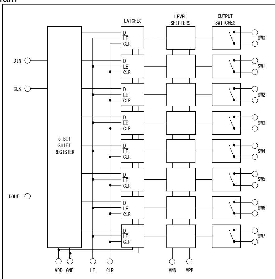
Fig. 1.3.1 Block diagram
