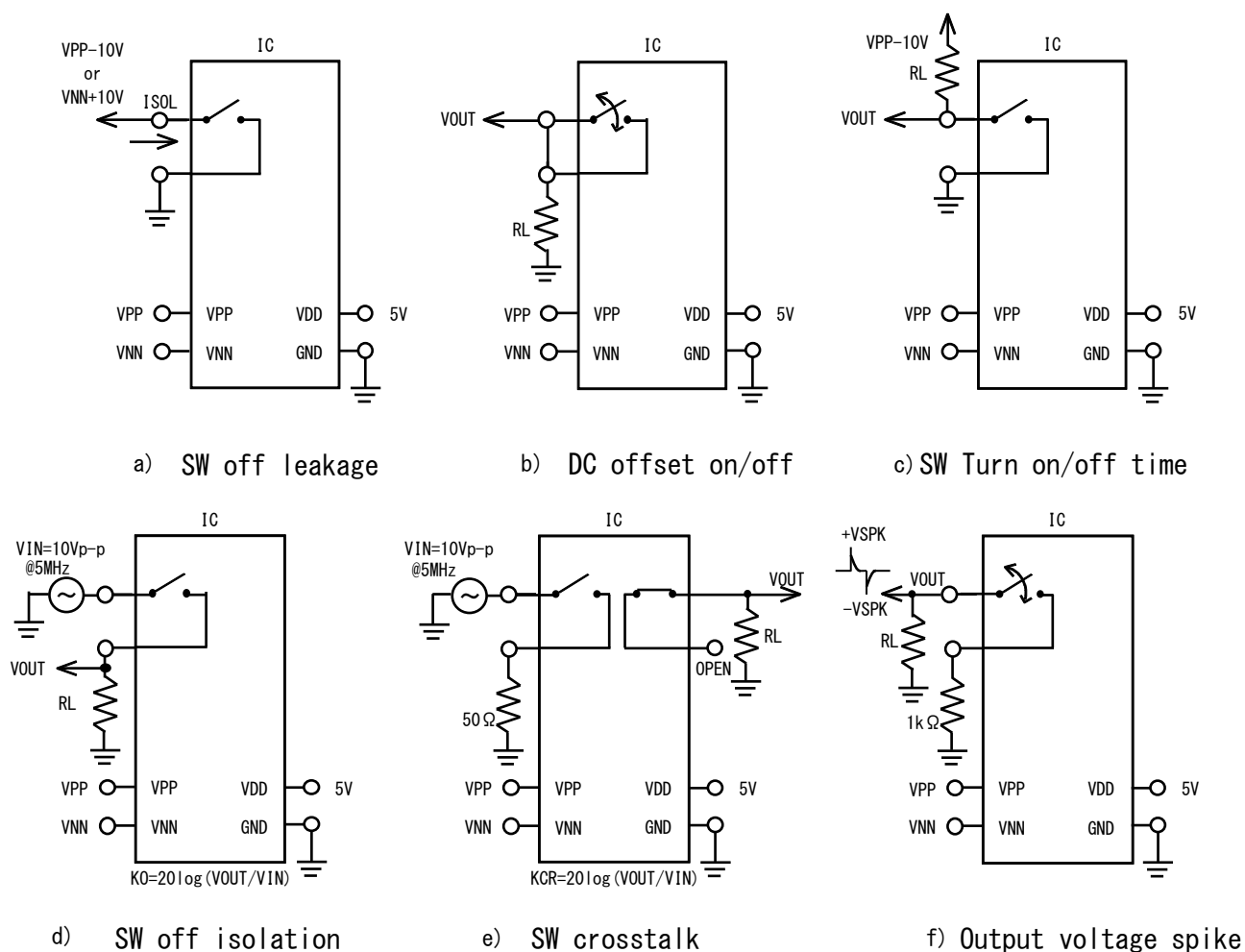
Fig. 4.1 Test Circuit
