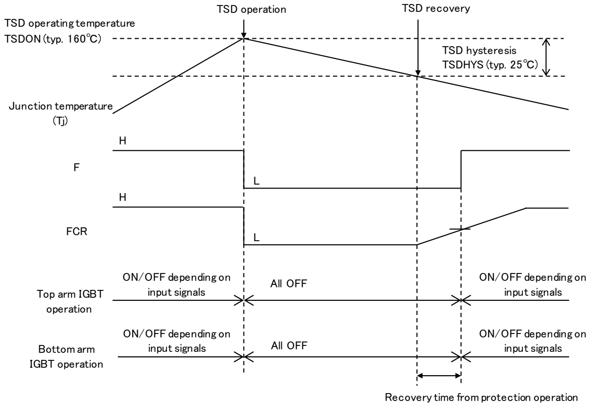
FIGURE 3.5.1.6 Timing Chart for Over Temperature Protection Operation
