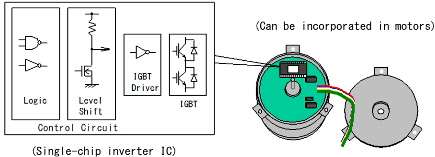
FIGURE 1.1.1 Image of Motor with Built-in Control Board
