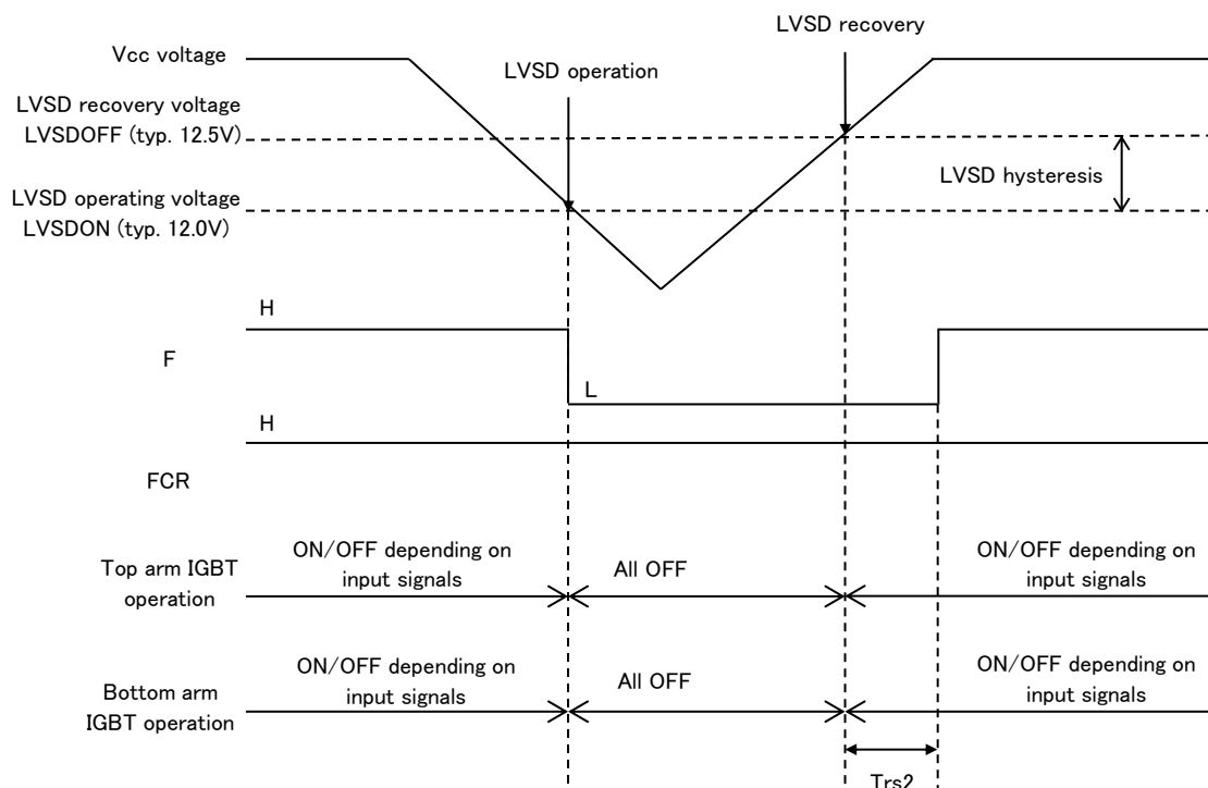
FIGURE 3.5.1.1 Timing Chart for Vcc Low-voltage Detection Operation
