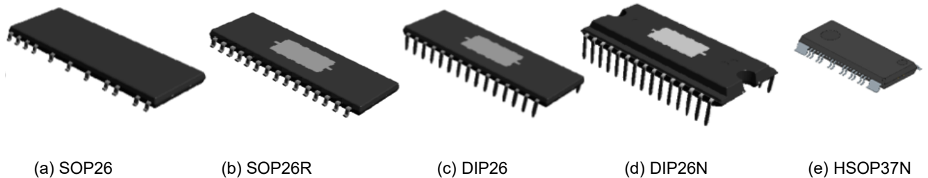
FIGURE 1.1.2 Types and Packages of IC
