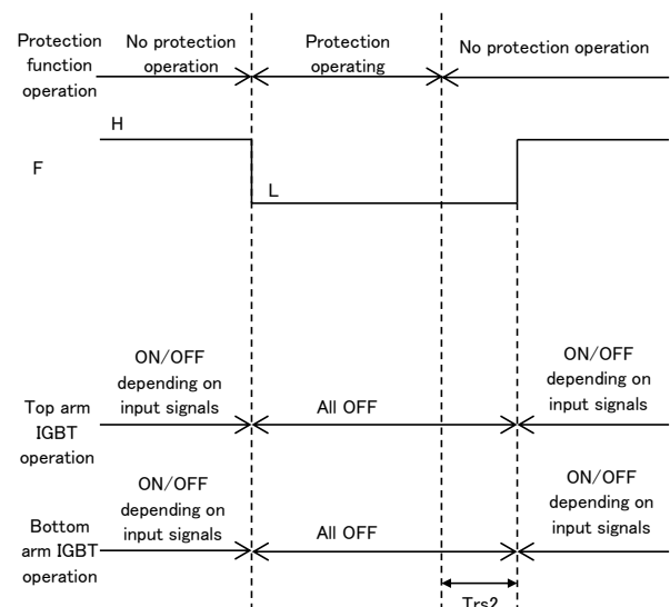
FIGURE 3.5.1.9 Timing Chart in Case of Protection Recovery Time Adjusting Function Disabled
