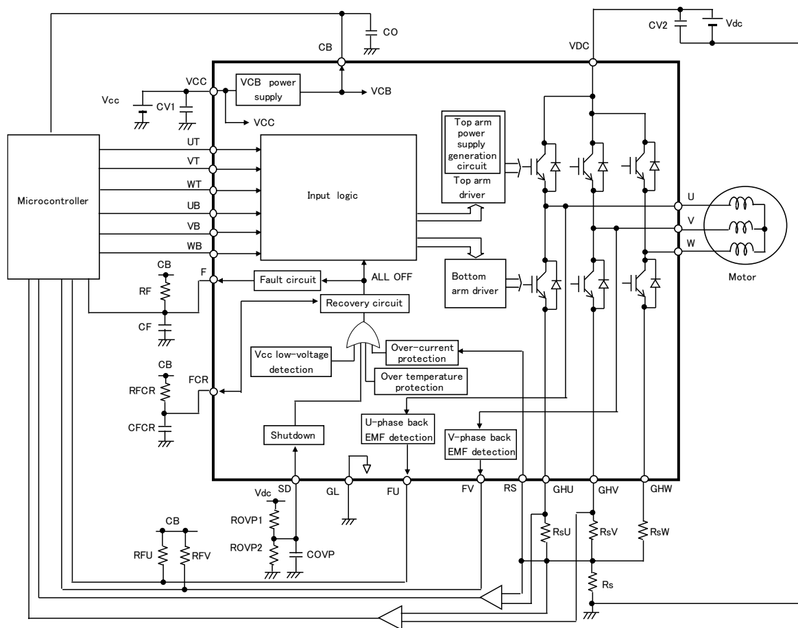
FIGURE 4.1.1 Block Diagram and External Components of IC
