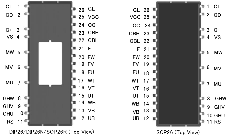
FIGURE 5.1 Pin Locations
