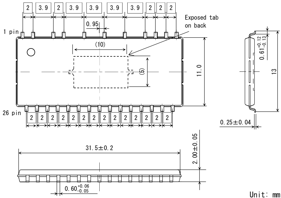
FIGURE B: Dimensions of SOP26
