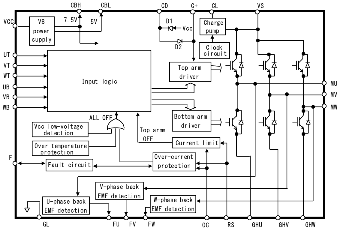
FIGURE 1.3.1 Block Diagram
