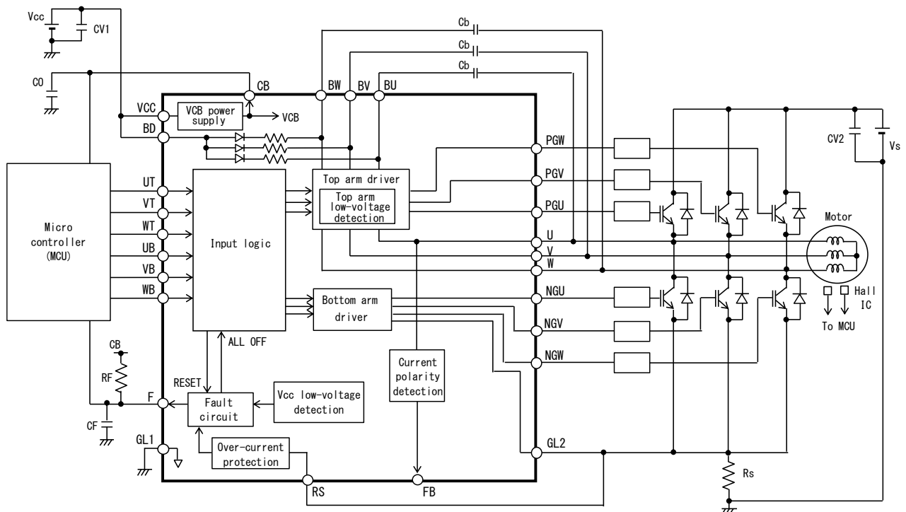
FIGURE 3.1.1 Block Diagram and External Components of IC
