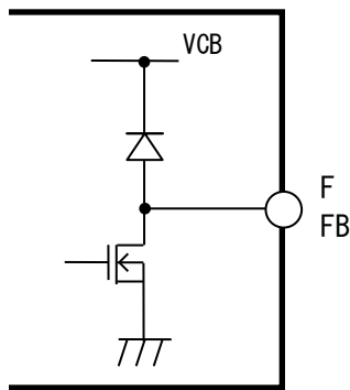
FIGURE 2.2.3 Equivalent Circuit Around F, FB Pins
