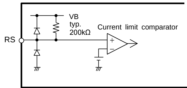
FIGURE 2.2.4 Equivalent Circuit Around RS Pin
