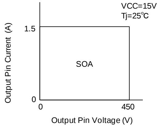
FIGURE 4.1.1 SOA
