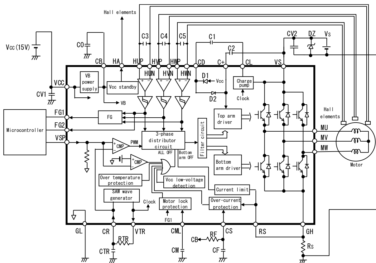
FIGURE 3.1.1 Block Diagram (ECN30210S is shown inside the bold line.)
