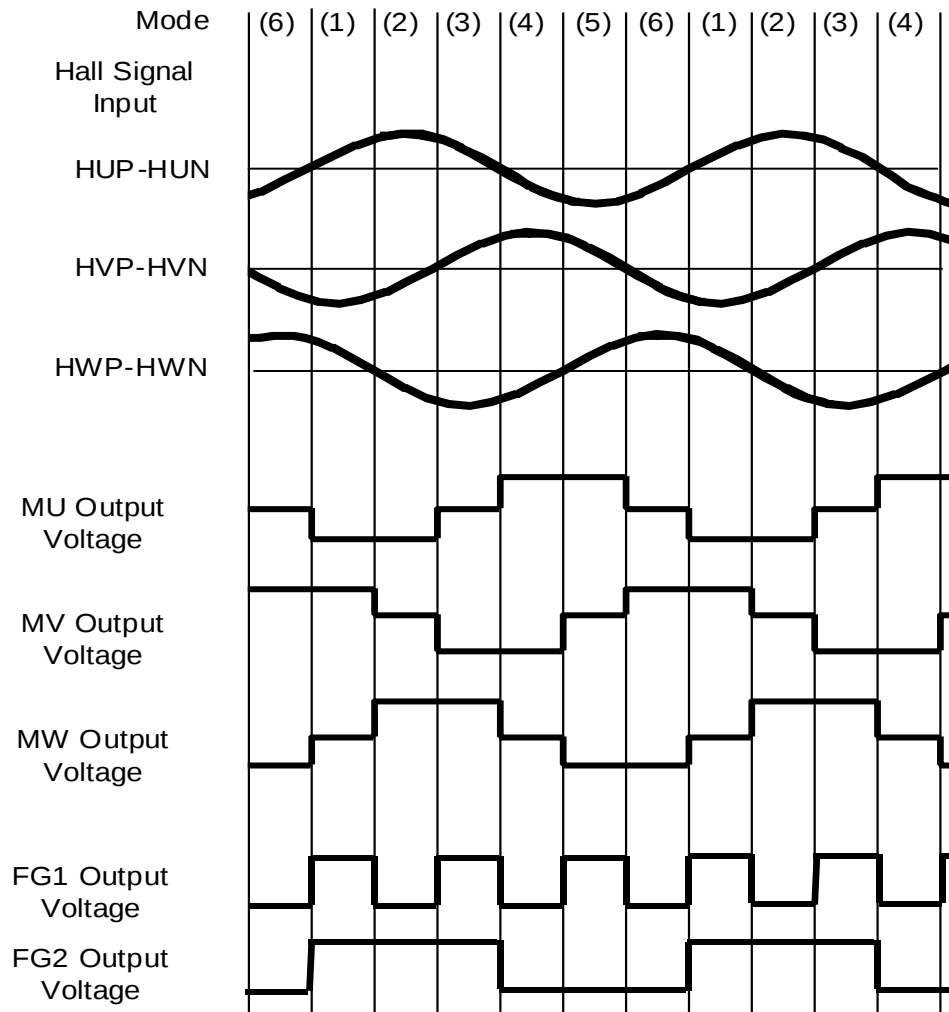
FIGURE 2.4.2.1 Timing Chart
