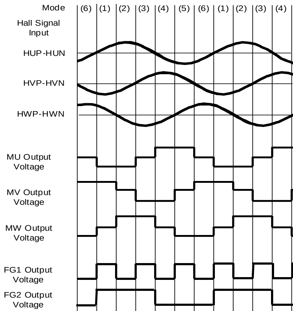
FIGURE 2.4.2.1 Timing Chart
