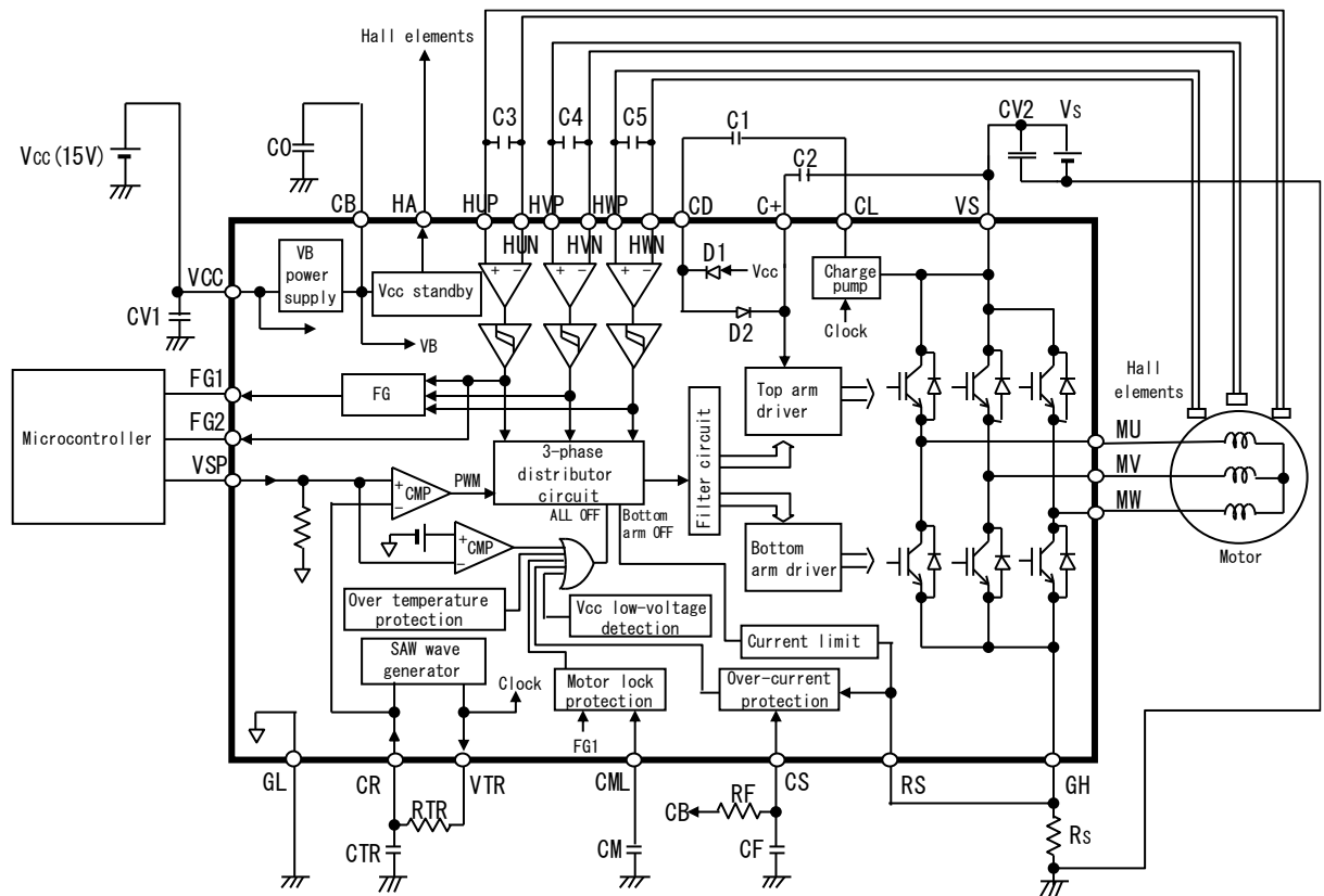
FIGURE 1.3.1 Block Diagram
