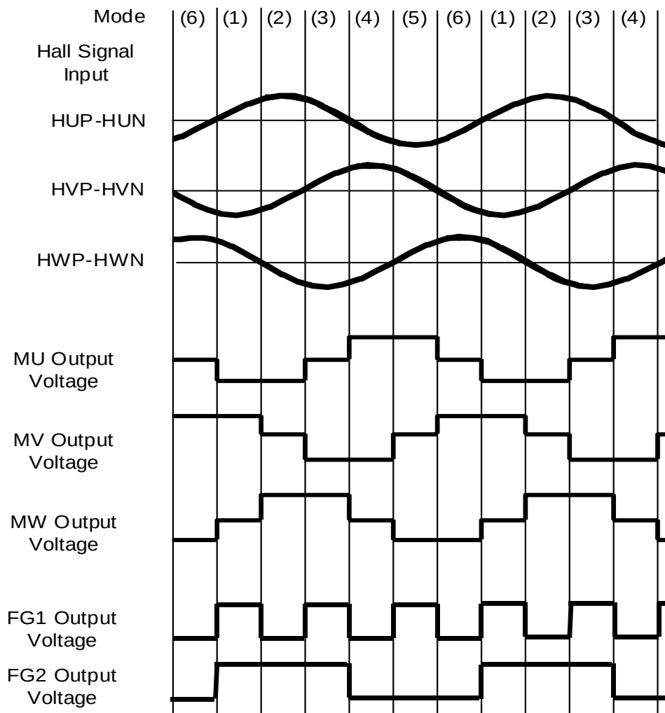
FIGURE 2.4.2.1 Timing Chart
