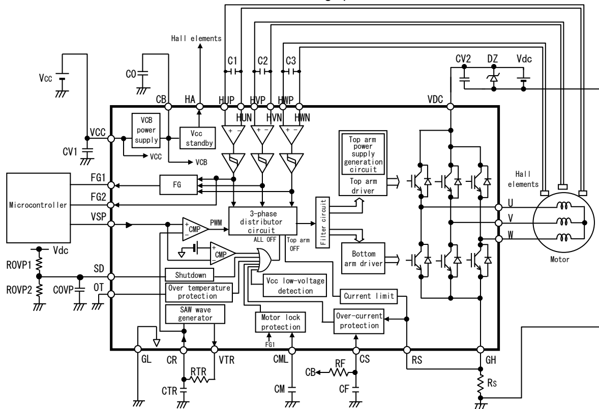
FIGURE 3.1.1 Block Diagram and External Components of IC
