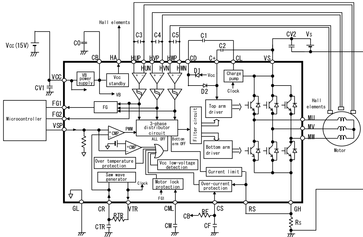
FIGURE 1.2.1 Block Diagram of Inverter IC
