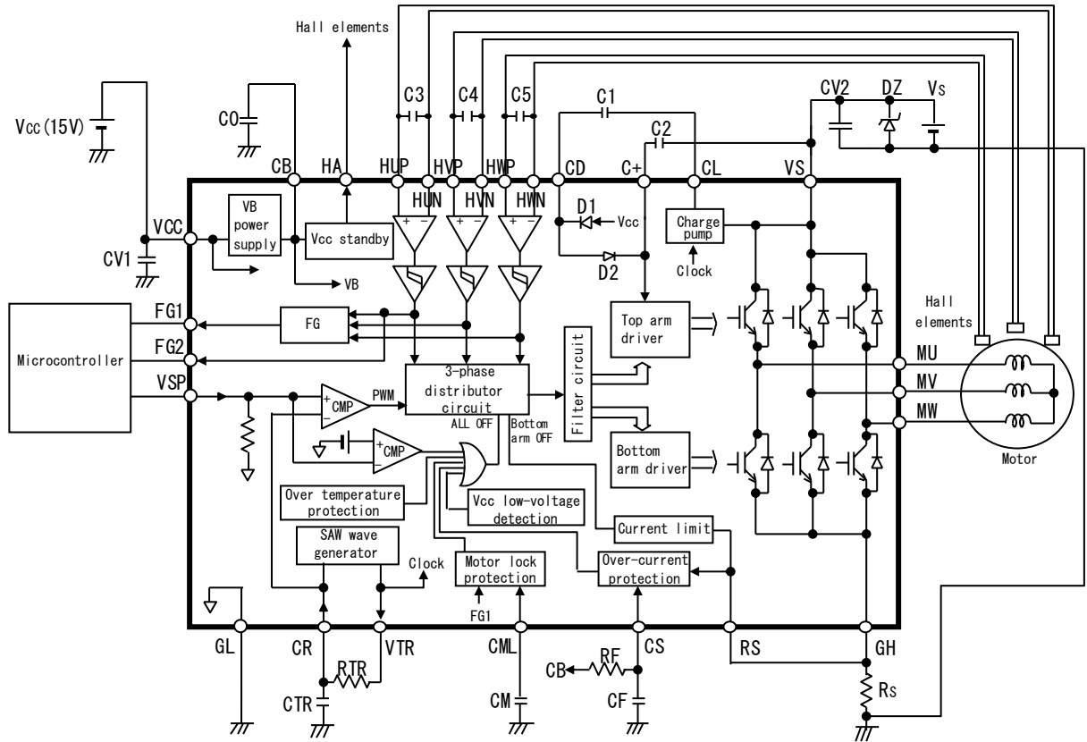
FIGURE 1.3.1 Block Diagram
