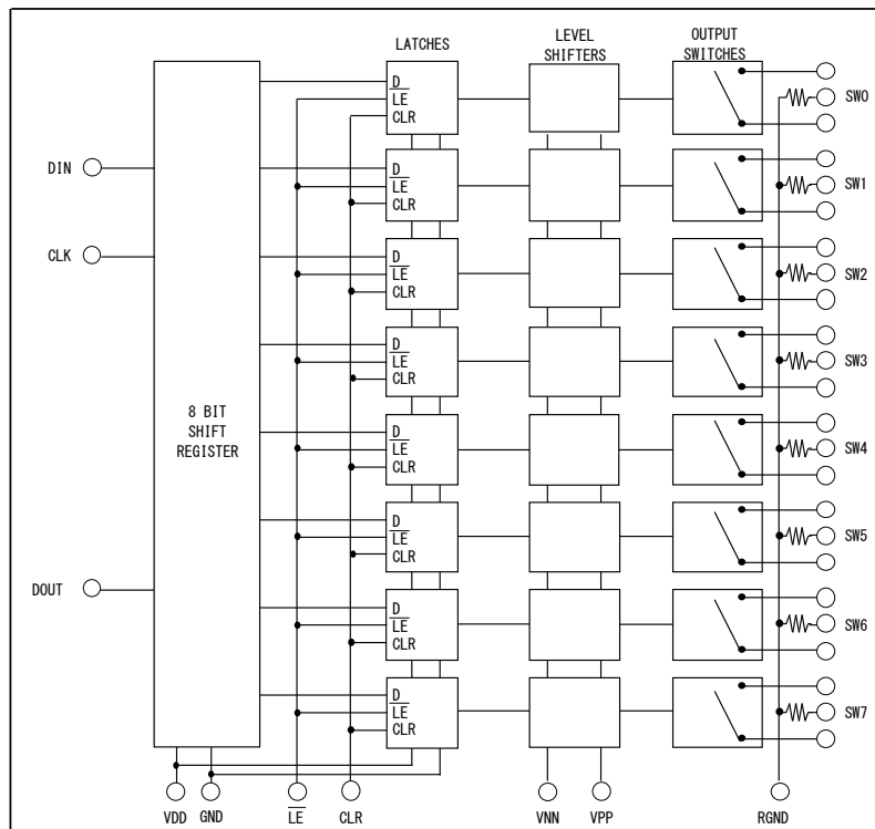
Fig. 1.3.1 Block diagram
