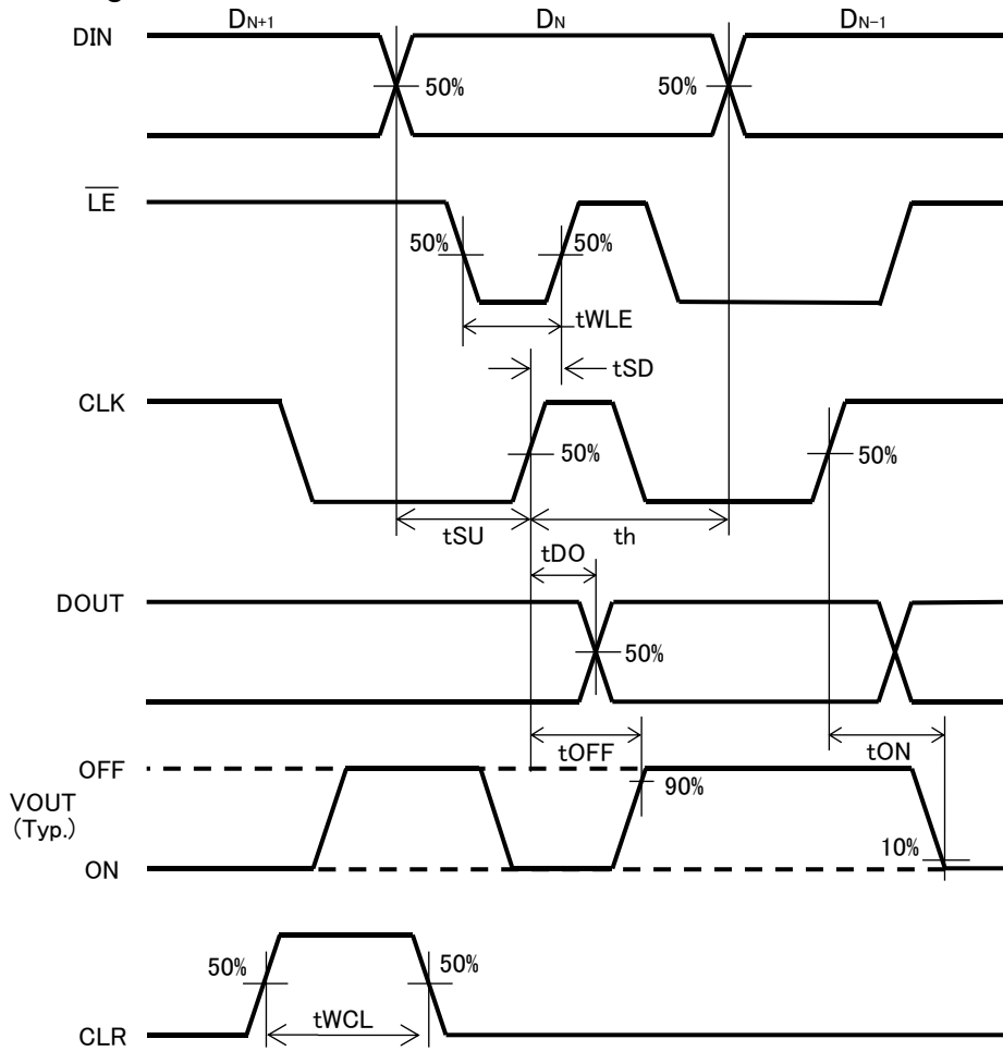
Fig. 5.1 Timing Waveforms
