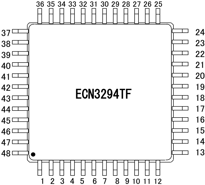
Fig. 8.1 Pin configuration(Top view)
