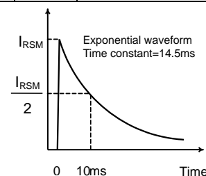
Figure 1. I_{RSM} waveform
