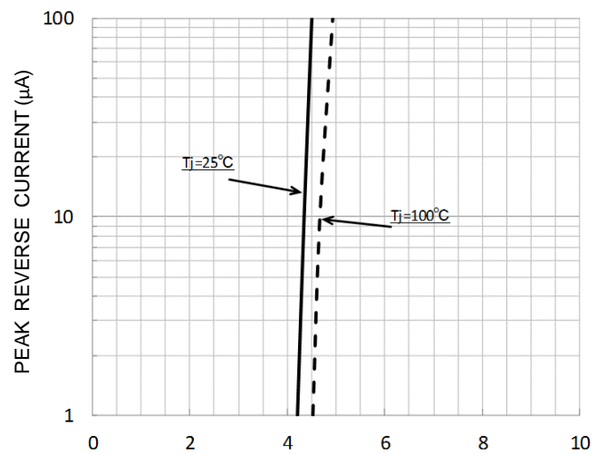
Typical Reverse Current characteristic ( I_r : 1\mu\text{A} \sim 100\mu\text{A} )
