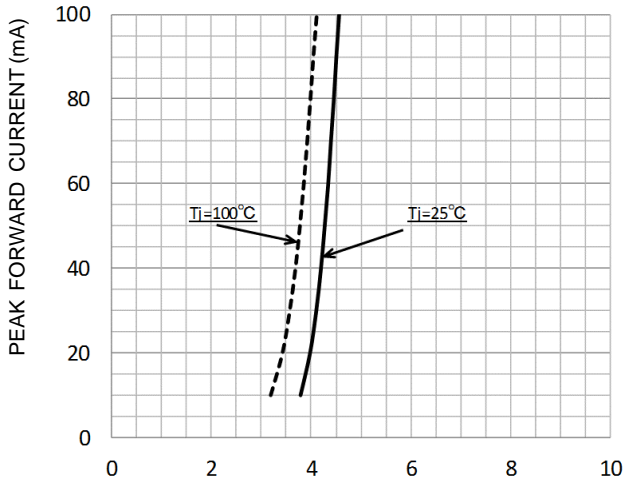
PEAK FORWARD VOLTAGE DROP (V)
