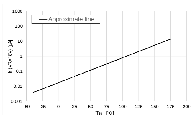
Fig.A-3. Leakage current – Temperature *
