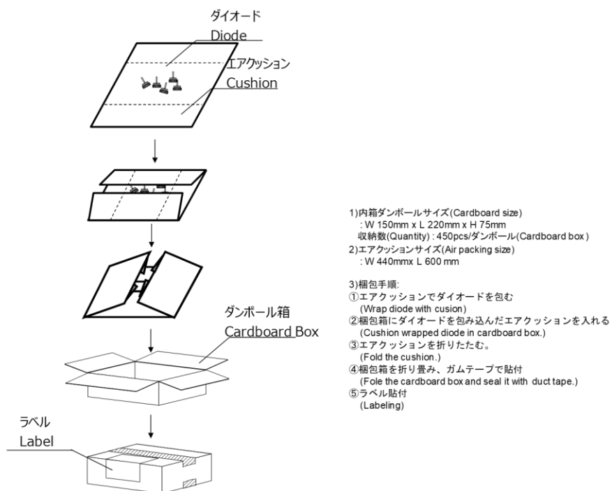
Fig7-2. Packing specification
