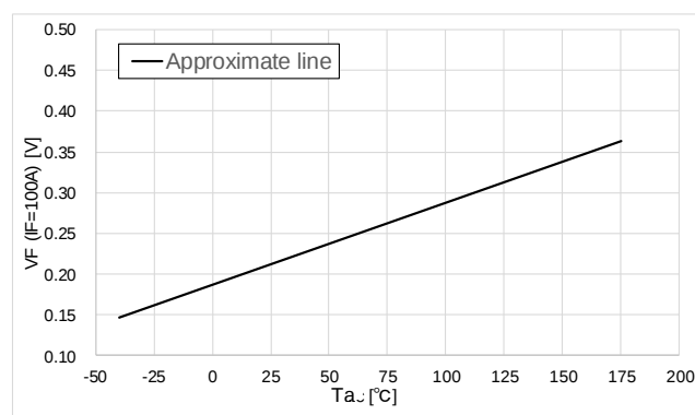
Fig.A-4. Forward voltage – Temperature *
