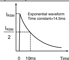
Figure 1. I_{RSM} waveform
