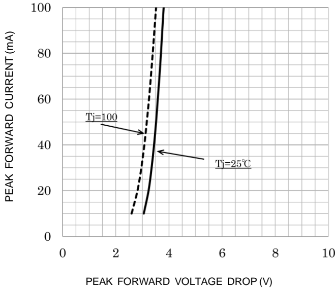
順特性 (代表例) Typical Forward characteristic
