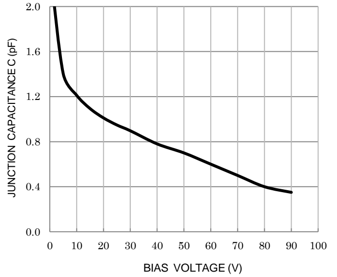
接合容量特性 (代表例) Typical Junction Capacitance
