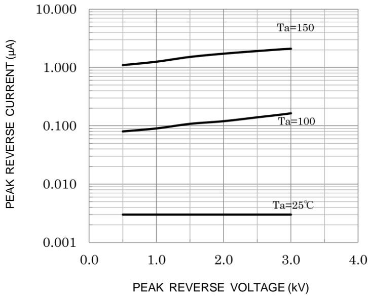
逆特性 (代表例) Typical Reverse Current characteristic ( I_r : 0.001\mu\text{A} \sim 10\mu\text{A} )
