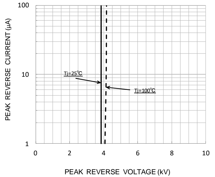
逆特性 (代表例) Typical Reverse Current characteristic ( I_r : 1\mu\text{A} \sim 100\mu\text{A} )
